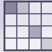
Activity Visualizer
