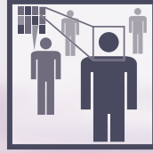
Face Collector
