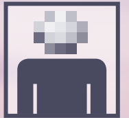
Privacy Protector
